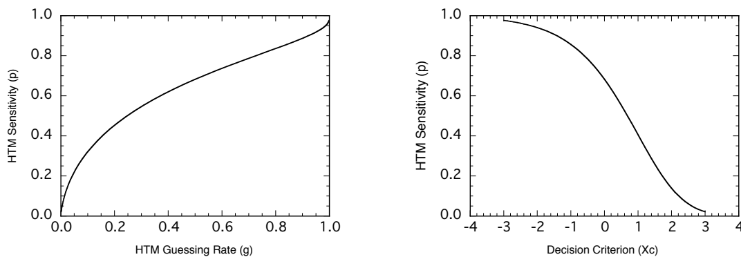
Figure 6: Sensitivity, p , of HTM sensory process computed from HR and FAR in the "yes-no" paradigm as a function of the guessing rate g (left panel) or the decision criterion, X_c (right panel). The High Threshold Model predicts that p should remain constant.
